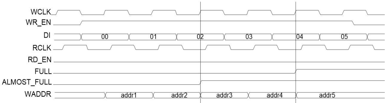
Figure 7-9 Write Timing to Almost Full Asynchronous FIFO
