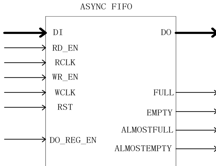
Figure 7-2 Asynchronous FIFO Mode (Without Rewrite/Resend Function)
