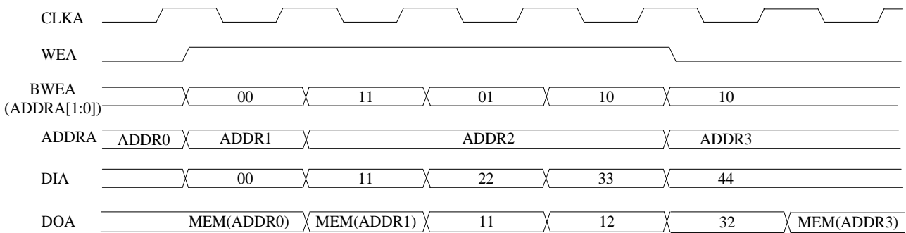
Figure 3-5 Byte Enable Read/Write Timing Diagram (TW Mode)
