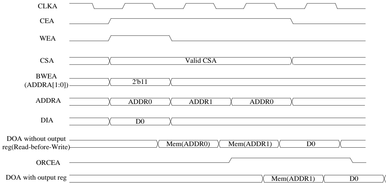
Figure 3-4 Read before Write Mode Read-Write Timing Diagram
