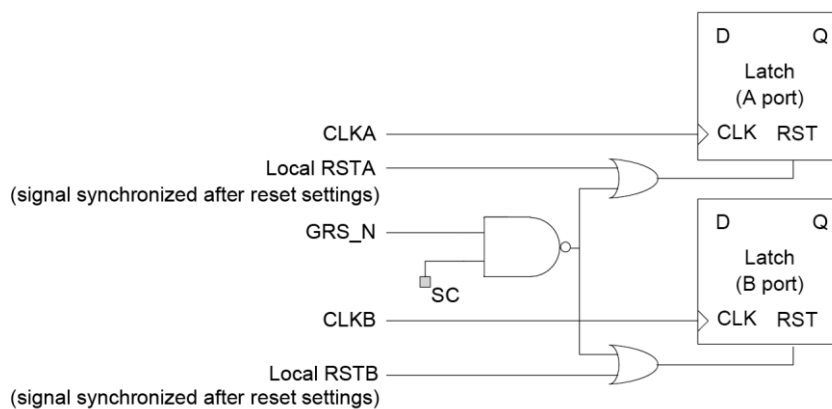
Figure 3-11 Core Reset
